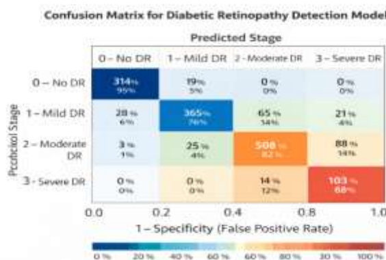
FIG 3.CONFUSION MATRIX
